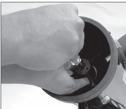
Figure 13. To center the secondary mirror under the focuser, hold the secondary mirror holder in place with your fingers while adjusting the center screw with the Phillips head screwdriver. Do not touch the mirror's surface.
