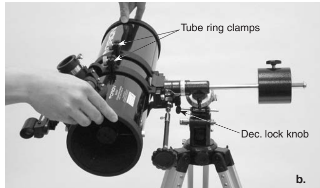
Figure 4. Proper usage of the equatorial mount requires the telescope tube to be balanced on both the R.A. and Dec. axes. (a) With the R.A. lock knob released, slide the counterweight along the counterweight shaft until it just counterbalances the tube. When you let go with both hands, the tube should not drift up or down. (b) With the Dec. lock knob released, loosen the tube ring lock clamps a few turns and slide the telescope forward or back in the tube rings. When the tube is balanced about the Dec. axis, it will not move when you let go.
